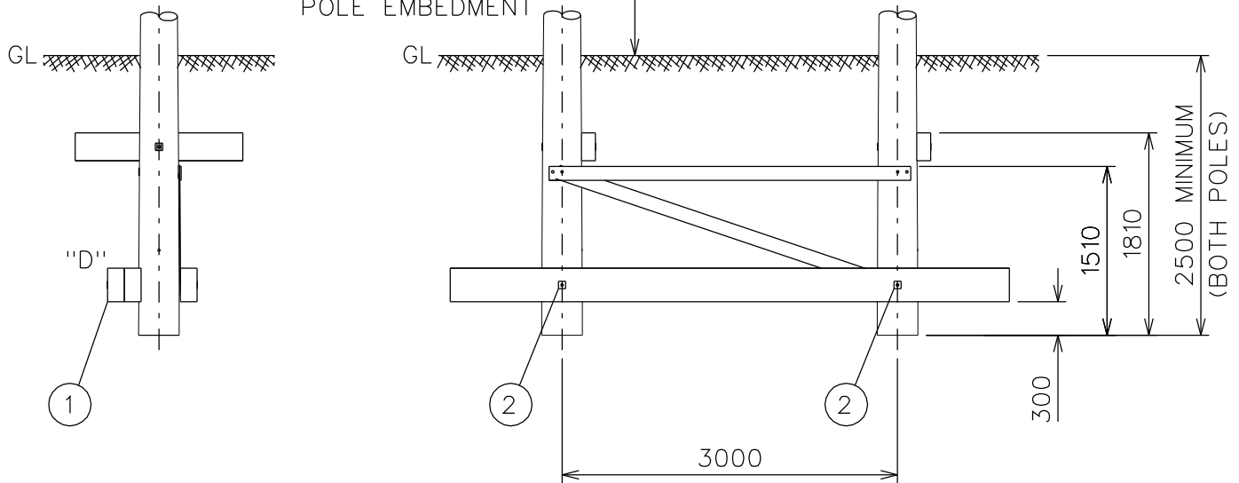
SIDE VIEW
